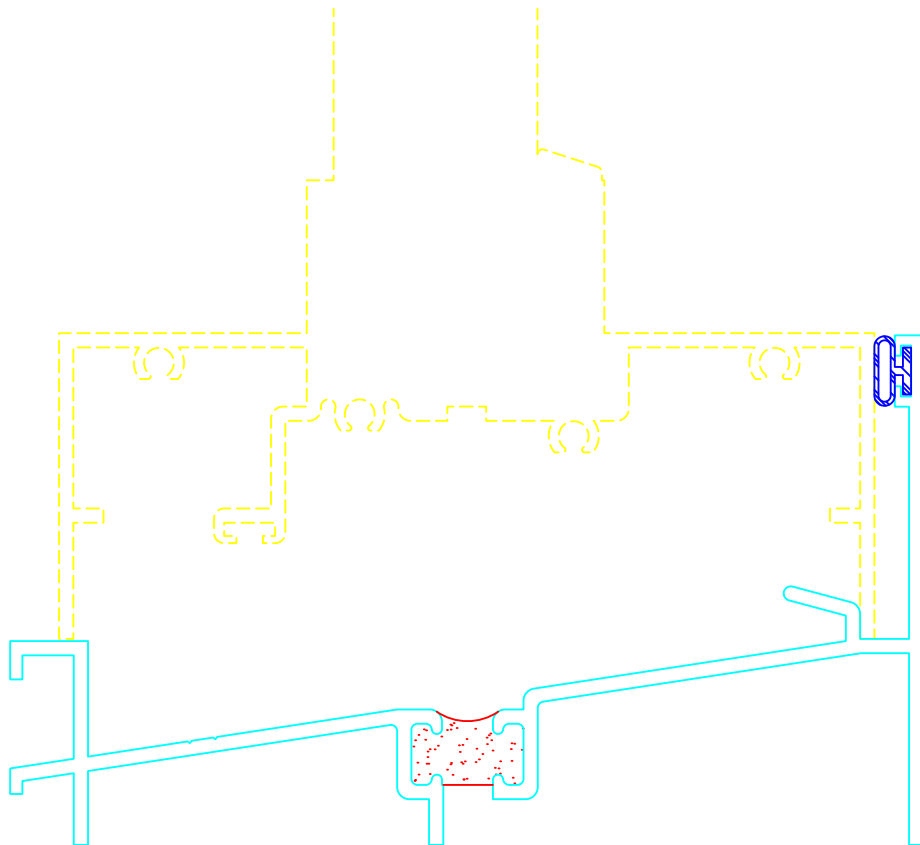
SUB SILL FULL SIZE
