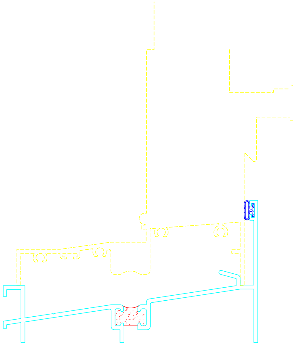
SUB SILL FULL SIZE
