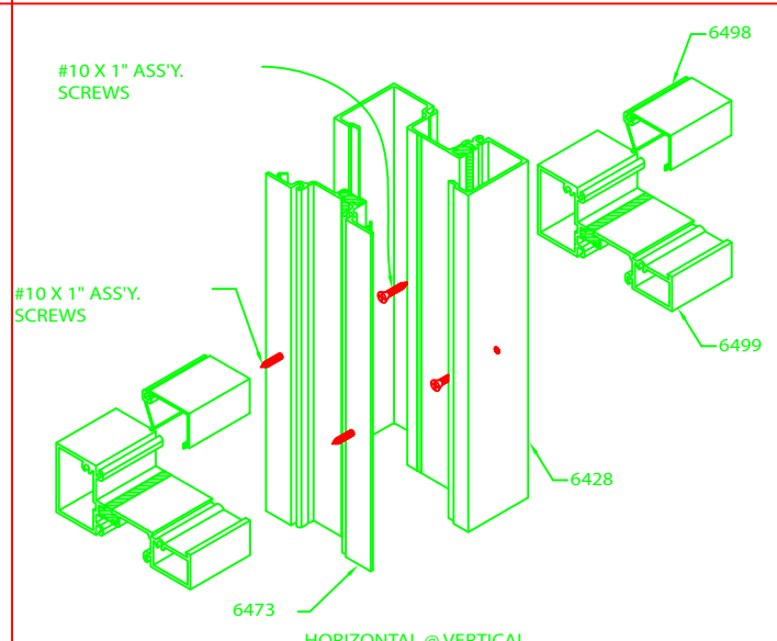
HORIZONTAL @ VERTICAL
