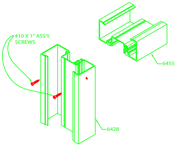
HEAD @ JAMB
