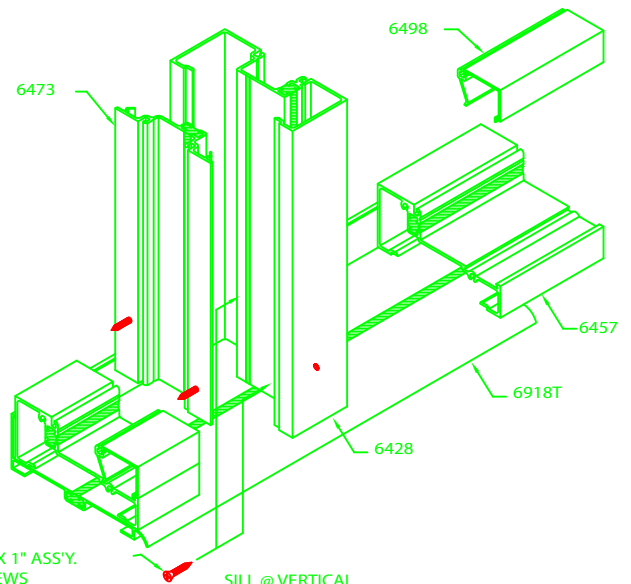
SILL @ VERTICAL
