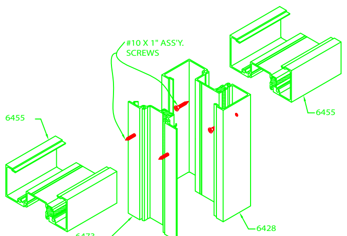
HEAD @ VERTICAL
