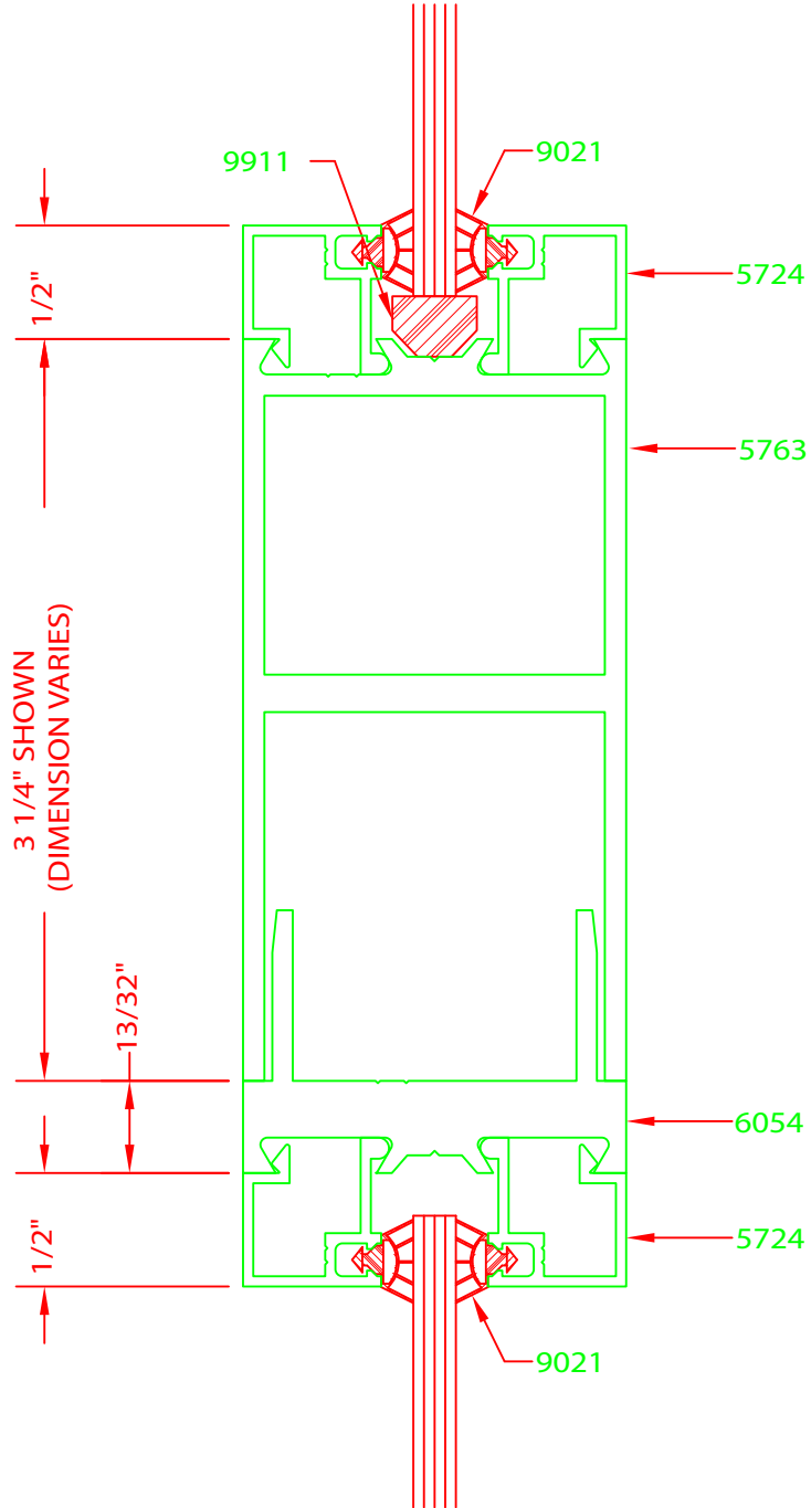
MUNTIN BAR (OPTIONAL)
